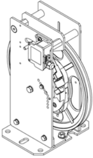
Fig. 1 Overspeed governor type LK120/LX120/LX150/LX180/ LX200/ LK200/LK250/LK300 /LK315 without remote control
