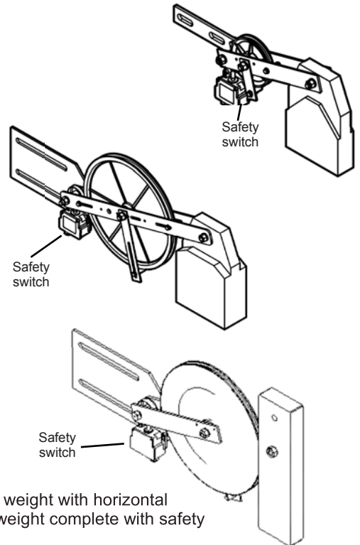
Fig. 3 Overspeed governor type LK120/LX120/LX150/LK180/ LX200/ LK200/LK250/LK300 /LK315 with uncontrolled car movement device
