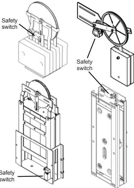
Fig. 5 Tension weight with vertical counterweight complete with safety switch
